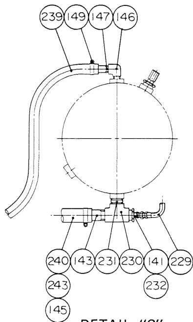
DETAIL "C"
