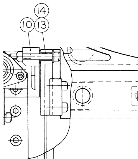
DETAIL "B"
